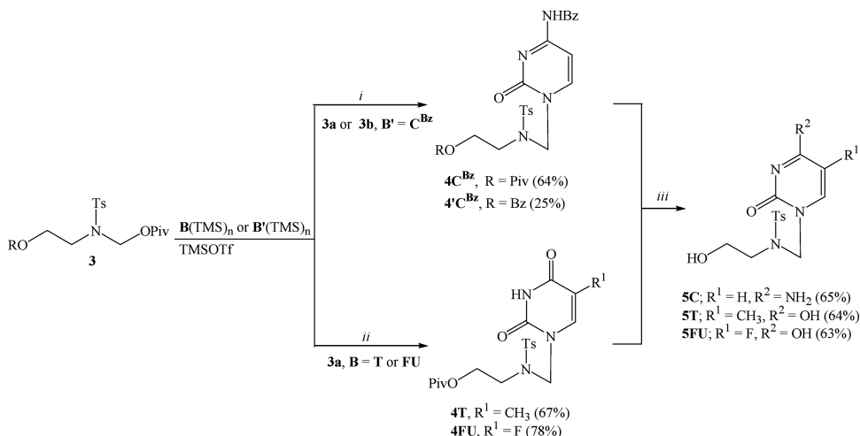
SCHEME 2 Reagents and conditions: (i) a) \text{C}^{\text{Bz}} , BSA, MeCN, rt, 1 hour; b) 3a or 3b , TMSOTf, MeCN, rt, 3 days; (ii) a) T or FU , BSA, MeCN, rt, 1 h; b) 3a , TMSOTf, MeCN, rt, 3 days; (iii) NH 3 aq/MeOH, 70°C, 5 days.
