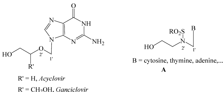
FIGURE 1 The general structure of aza-analogues of Acyclovir ( A ).
