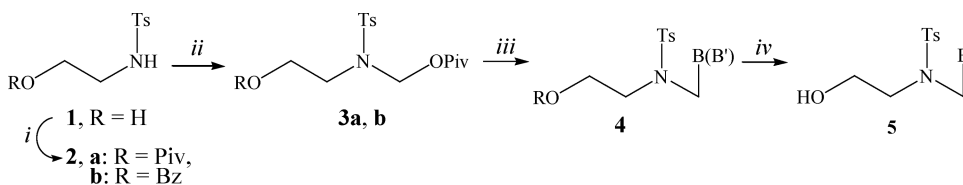
SCHEME 1 Reagents and conditions: ( i ) BzCl or PivCl, Py, rt, 1 day ( 2a , 90%; 2b , 91%); ( ii ) PivOCH 2 Cl, K 2 CO 3 , DMF, rt, 5 days ( 3a , 85%; 3b , 80%); ( iii ) B(TMS) n or B'(TMS) n , Lewis acid; ( iv ) NH 3 aq/MeOH.
